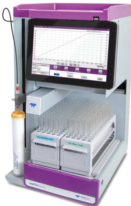
Figure 1-1 CombiFlash NextGen 100 with 12 inch display, 1-100 mL/min, 150 psi (without solid load injection valve)
