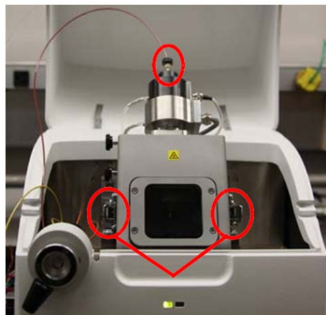
Figure 5-11 ESI and APCI removal from PurIon S and PurIon L
