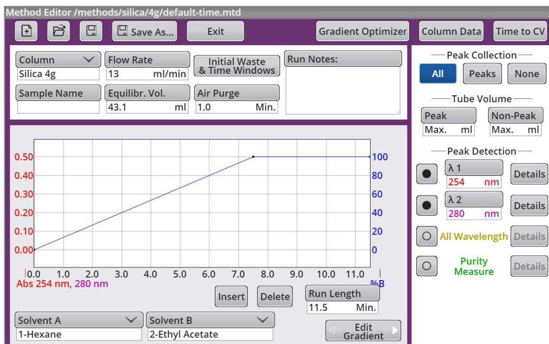
Figure 3-4 METHOD EDITOR screen
