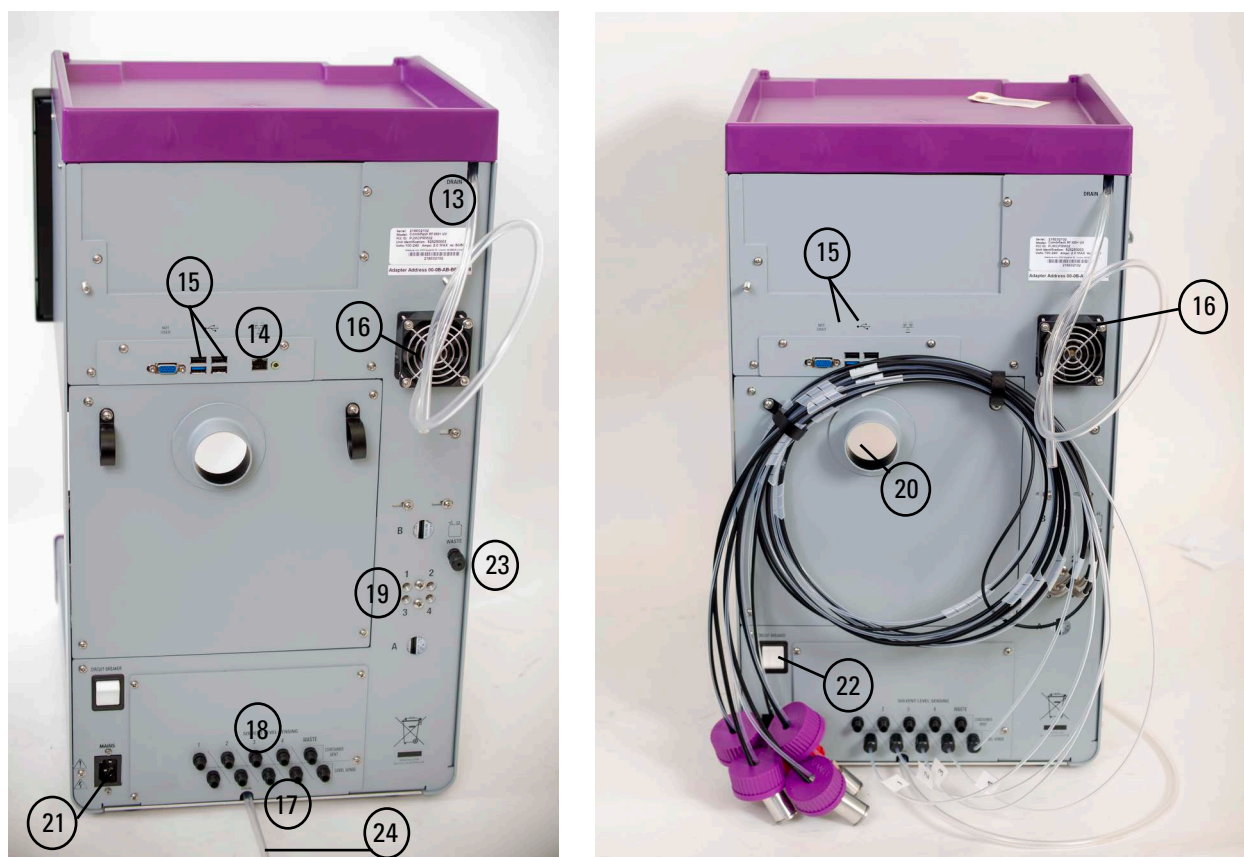
Figure 1-7 CombiFlash NextGen features (back)
