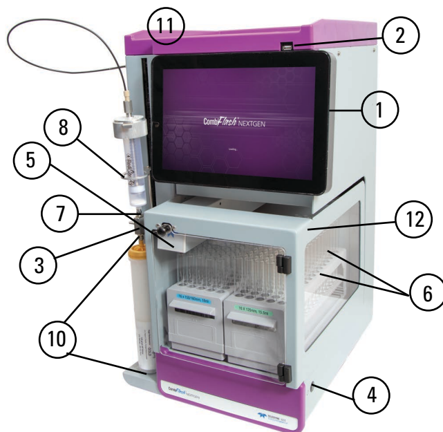
Figure 1-5 CombiFlash NextGen features (front)
