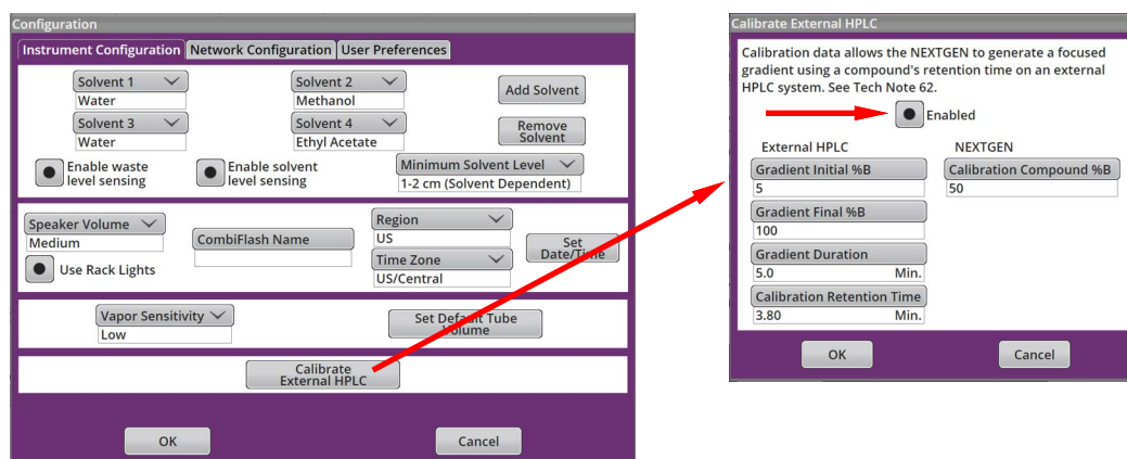
Figure 3-22 Opening the Calibrate External HPLC window from the Configuration window
